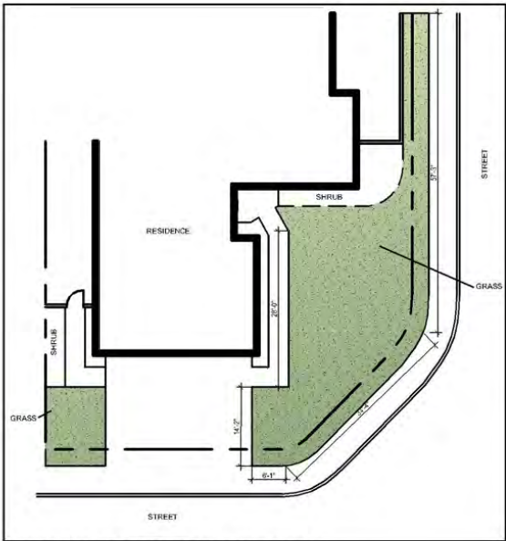
EXISTING CONDITIONS DIAGRAM
