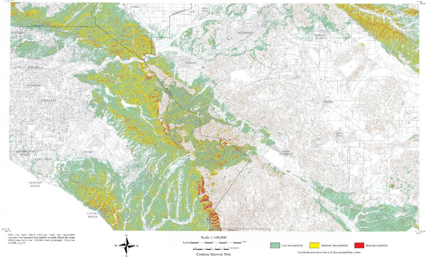
Plate 5. Soil-Slip Susceptibility Map for the Santa Ana 30' x 60' Quadrangle, Southern California Preliminary Soil-Slip Susceptibility Maps, Southwestern California
